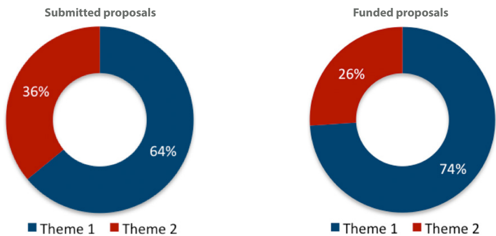
Fig. 6: Proportion of the proposed research themes between submitted and funded proposals. One proposal can address several themes.
